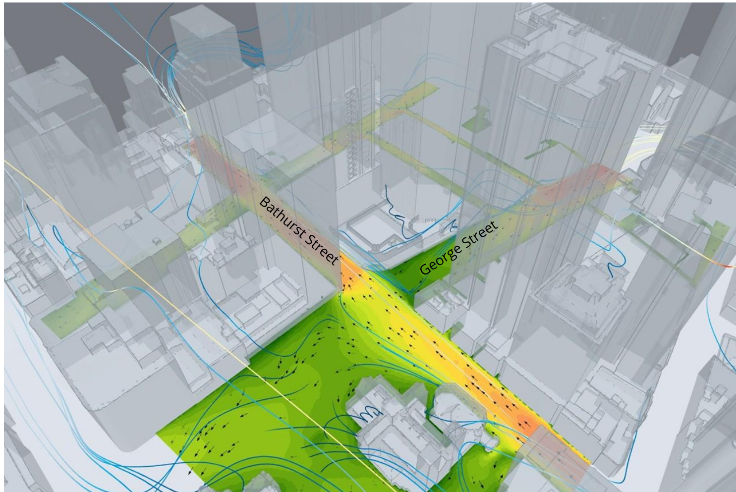
Image 8c: Interaction of Prevailing West Winds with Existing Building Winds from 270° sector
