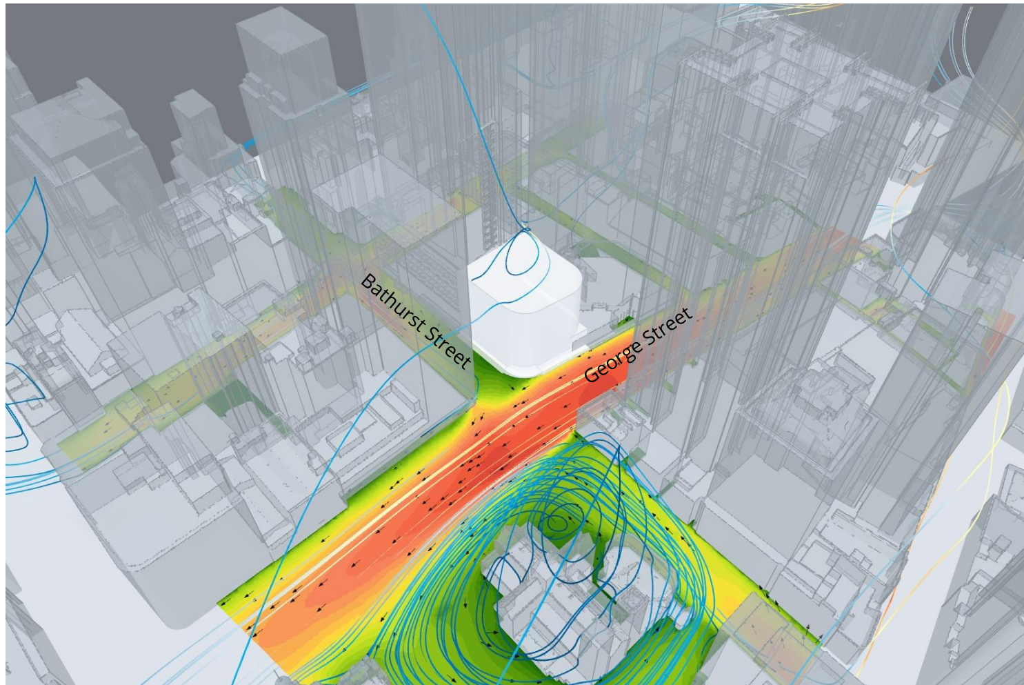
Image 8e: Interaction of Prevailing South Winds with Indicative Design Massing Winds from 180° sector
