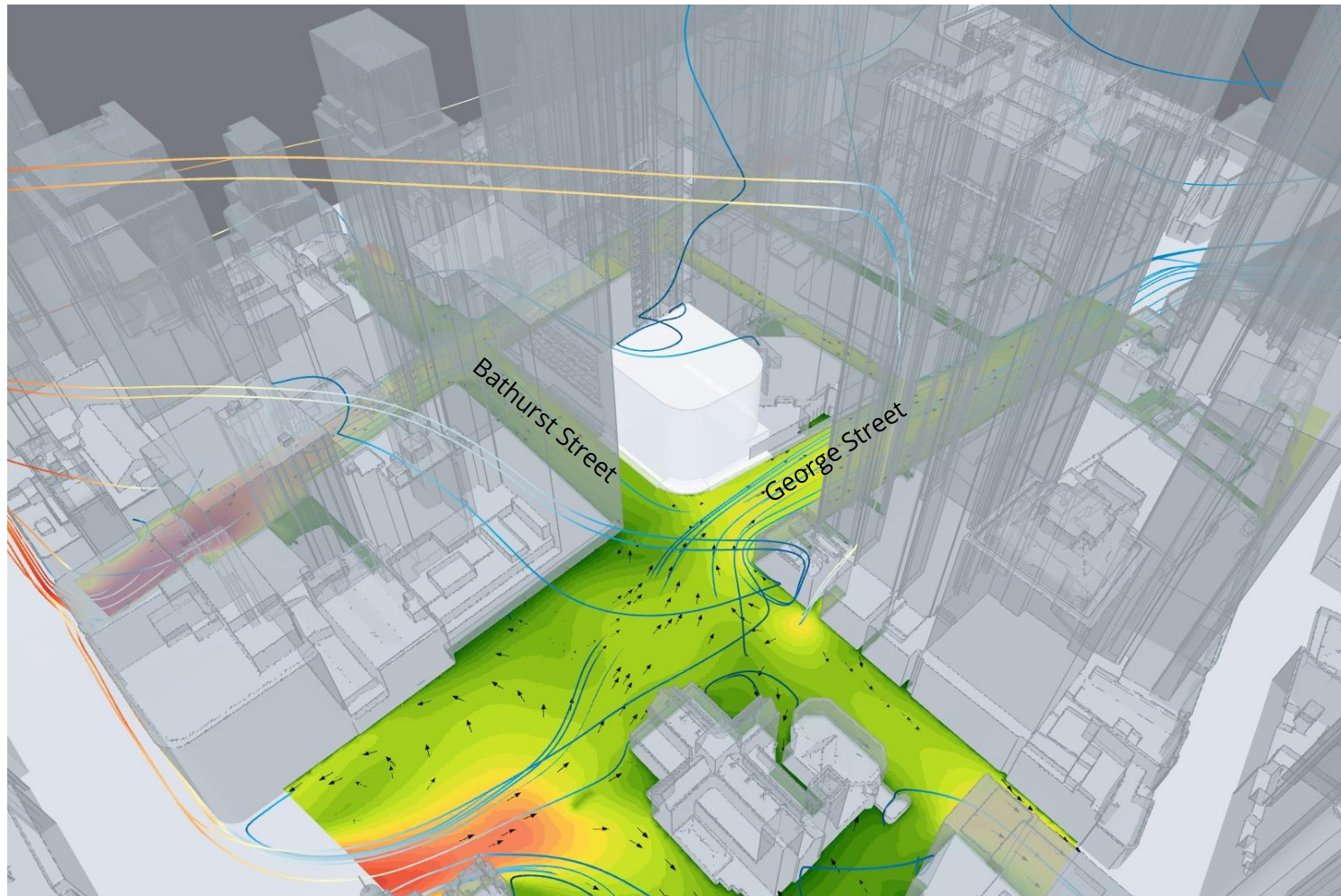
Image 8d: Interaction of Prevailing Northeast Winds with Indicative Design Massing Winds from 45° sector
