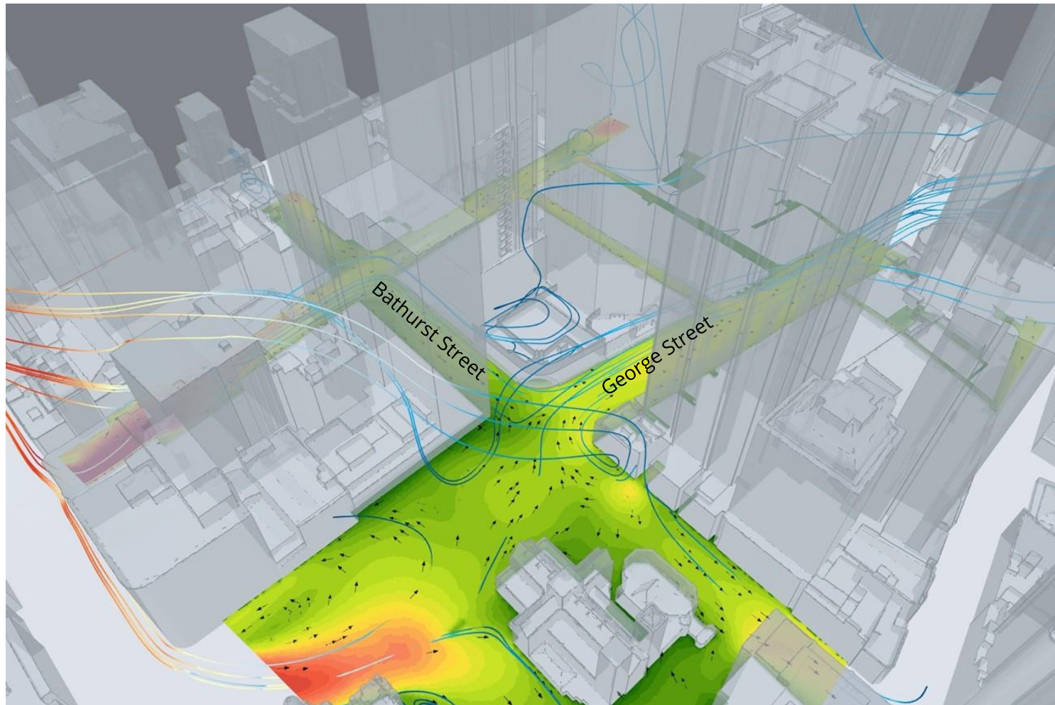
Image 8a: Interaction of Prevailing Northeast Winds with Existing Building Winds from 45° sector
