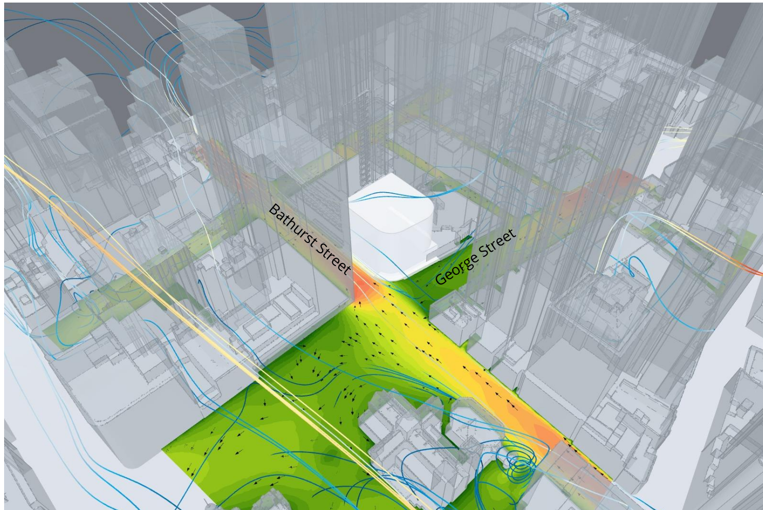
Image 8f: Interaction of Prevailing West Winds with Indicative Design Massing Winds from 270° sector
