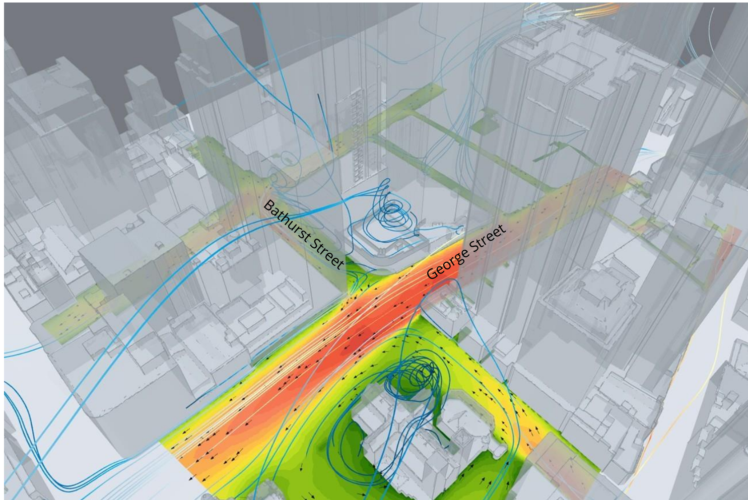
Image 8b: Interaction of Prevailing South Winds with Existing Building Winds from 180° sector
